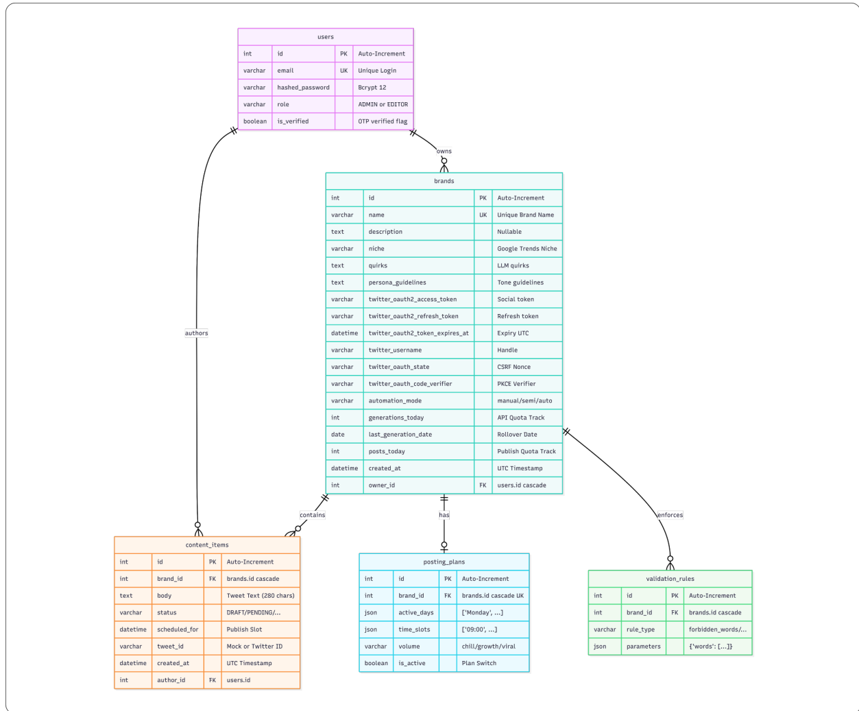
Figure 3.2: Relational Schema Entity-Relationship Diagram (ERD)
